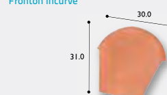
Tapa de caballate curvo Curved ridge end cap Fronton incurvé
