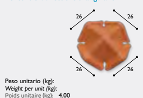
Caballete a 4 aguas triangular Triangular 4 ridge junction Rencontre 4 directions triangulaire
